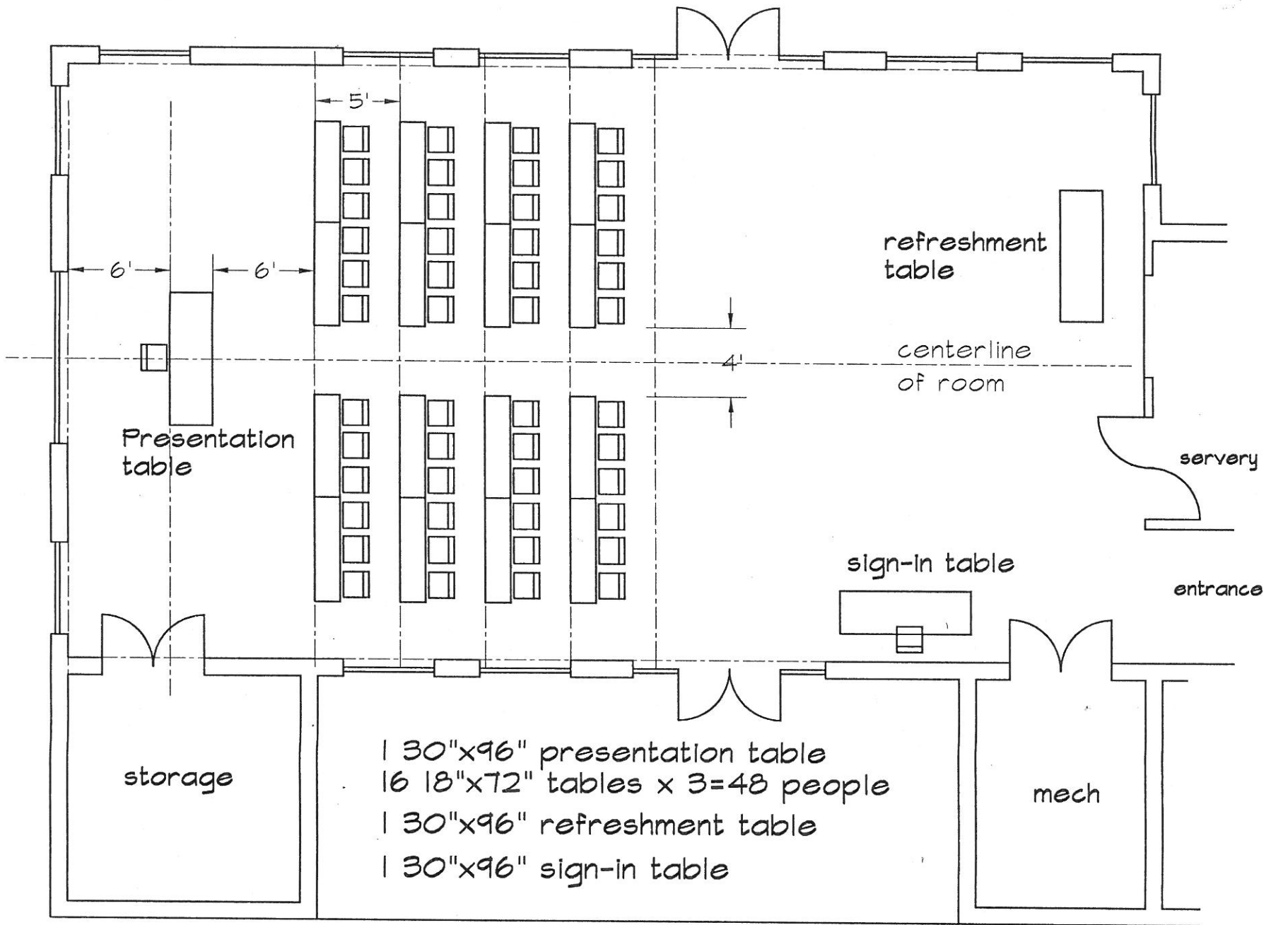
ROOM LAYOUT #3
